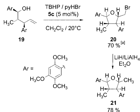
Scheme 1. Formation of 2- epi -magnosalicin ( 21 ) from 2-methyl-1,3-bis(2,4,5-trimethoxyphenyl)-4-penten-1-ol ( 19 )
