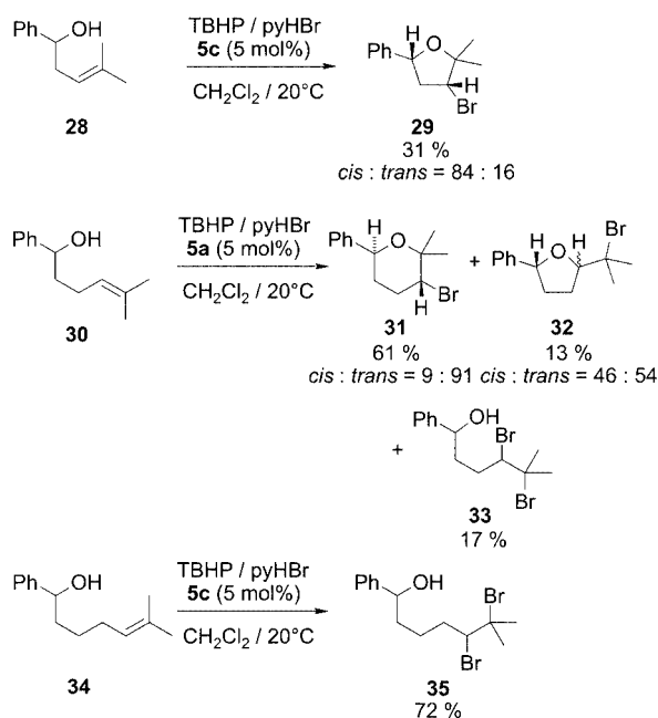
Scheme 3. The conversion of \omega,\omega -dimethyl-1-phenyl-substituted alkenols 28 , 30 , and 34 into brominated compounds
