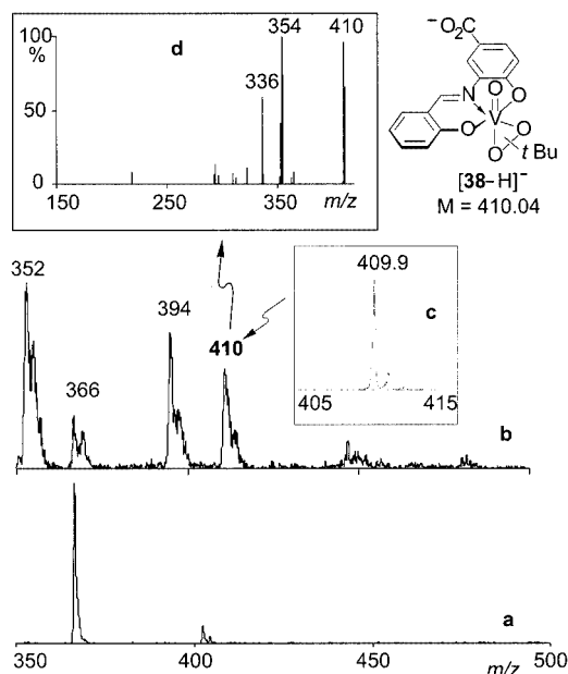
Figure 6. Identification of (Schiff base)vanadium(v) peroxy complex [38 - H] - by ESI-MS; insets: (a) full-scan spectrum of complex 5h (negative ions; solvent: CH 2 Cl 2 /CH 3 CN); (b) full-scan spectrum 30 min after treatment of complex 5h with TBHP; (c) zoom-scan spectrum showing the molecular ion [M - H] - of peroxy complex 38 ; (d) fragmentation (CID spectrum) of the isolated parent ion at m/z = 410
