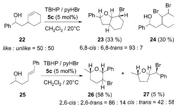
Scheme 2. Formation of bromination products from 5-substituted bis(homoallylic) alcohols 22 and 25
