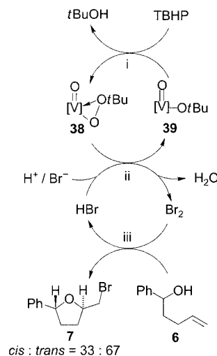
Scheme 6. Schematic presentation of reaction cycles leading to the formation of 2-(bromomethyl)-5-phenyltetrahydrofuran ( 7 ) from TBHP, pyHBr, 1-phenyl-4-penten-1-ol ( 6 ), and vanadium(v) compounds 38 and 39 (data refer to reaction in \text{CHCl}_3 ); \text{O}=[\text{V}]^+ refers to the fragment \text{VOL}^+ , where \text{H}_2\text{L} represents a tridentate dibasic Schiff base auxiliary such as 4 .
