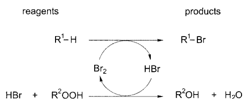
Figure 1. Principle for the in situ generation of Br 2 and its application in the synthesis of organobromine compounds; [1–4,7] R 1 = e.g. aryl; R 2 = H, alkyl
