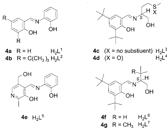
Figure 3. Structures of Schiff bases H 2 L 1 –H 2 L 7 ( 4a–g ) intended to serve as ligands for the syntheses of vanadium(v) complexes 5a–g (see Table 1) [16,19]
