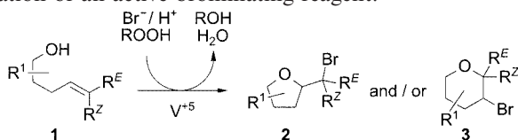
Figure 2. Strategy for the conversion of alkenols 1 in the presence of Br − , ROOH, and V 5+ into bromo-cyclized target products 2 and/or 3 ; R = H, C(CH 3 ) 3 ; R 1 = CH 3 , C 6 H 5 , aryl; R E = H, CH 3 , C 6 H 5 ; R Z = H, CH 3 ; V 5+ = (Schiff base)vanadium(v) complex, e.g. 5 (see Table 1)
