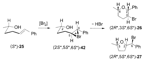
Scheme 8. Stereochemical model for the selective conversion of alkenol ( S * )- 25 into products (2 R * ,3 S * ,6 S * )- 26 and (2 R * ,5 S * ,6 S * )- 27 ; [Br 2 ] = TBHP, pyHBr, 5c
