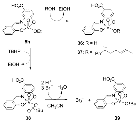
Scheme 4. Ligand exchange in the (Schiff base)vanadium(v) complex 5h : (i) formation of tert -butylperoxy complex 38 ( ^{51}\text{V} NMR spectroscopy and ESI-MS) and its reactivity towards bromide, and (ii) generation of complexes 36 and 37
