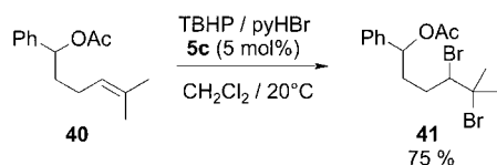
Scheme 5. Formation of dibromide 41 from olefin 40
