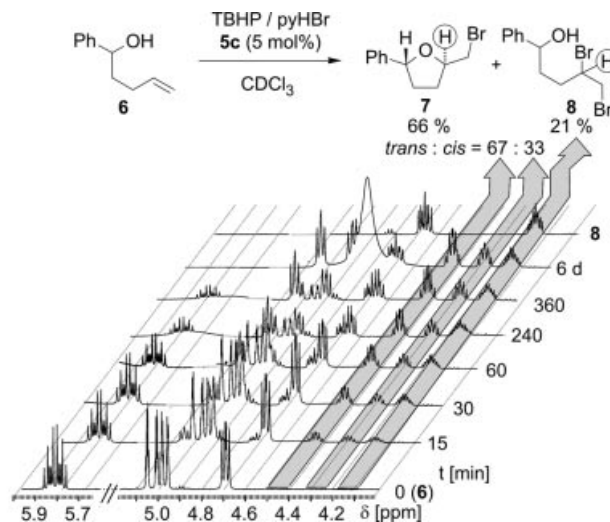
Figure 5. Stacking plot: time-dependent 1 H NMR study on the conversion of 1-phenyl-4-penten-1-ol ( 6 ) in the presence of TBHP (1.1 equiv.), pyHBr (1.5 equiv.), and methioninol-derived vanadium(v)-catalyst 5c (20 °C, CDCl 3 ); the selected spectral region depicts the resonances of olefinic protons, benzylic protons, and protons located in the vicinity of oxy or bromo substituents; for illustrative purposes the spectra of neat alkenol 6 and of purified dibromide 8 (equimolar mixture of like/unlike isomers) have been added to this plot
