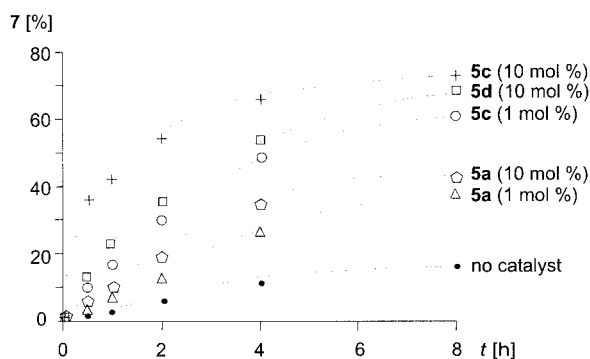
Figure 4. Time dependence of 2-(bromomethyl)-5-phenyltetrahydrofuran formation from 1-phenyl-4-penten-1-ol ( 6 ), TBHP, and pyHBr in the presence of vanadium(v) catalysts 5a , 5c , and 5d (CHCl 3 , 20 °C, GC)
